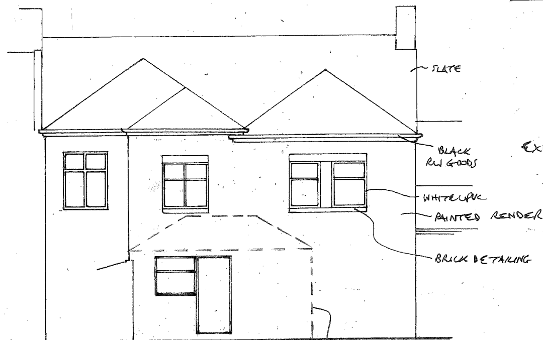
EXISTING REAR 1:100 EXISTING CONSERVATORY DEMOLISHED
